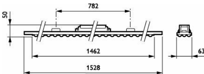
Maxos Led Industry - Generation 4 - 1 unit for TL-D 58 W - LED Module, system flux 5500 lm - 840 neutral white - Power supply unit with DALI interface - Wide beam - Connection unit 5-pole - White
