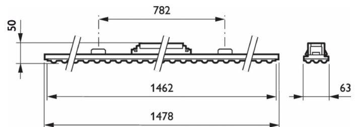
Maxos Led Industry - 1 unit for TL5 49 W - LED Module, system flux 5500 lm - 830 warm white - Power supply unit with DALI interface - Wide beam - Silver
