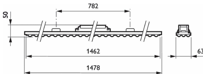
4MX850 491 LED55S/840 PSD WB SI
