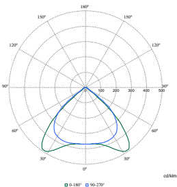
Polar Normal (separate) - 4MX400I - 910629123926
