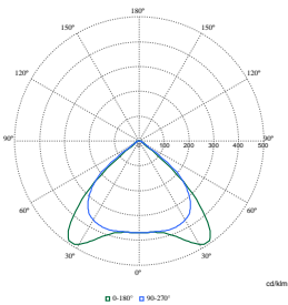
Polar Normal (separate) - 4MX400I - 910629123726
