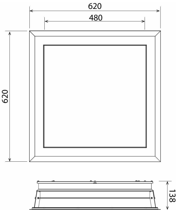
LP913P NC3 SKYLIGHT DIA W62L62
