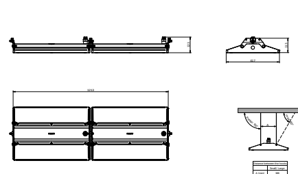
700s suspended
