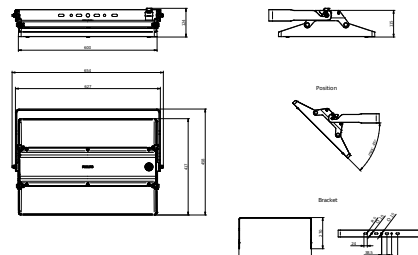
BY581P, BY583P Wallmounted bracket
