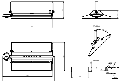
BY581X Bracket
