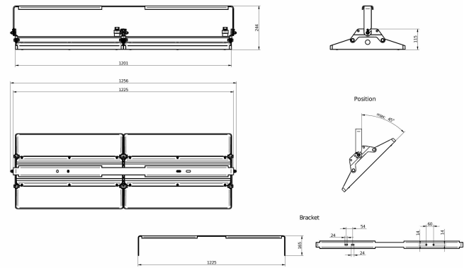
700S Bracket
