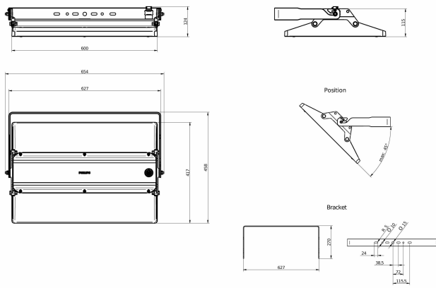
BY581P, BY583P Wallmounted bracket
