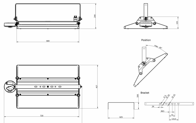
BY581X Bracket
