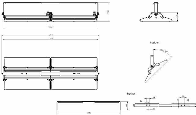
700S Bracket
