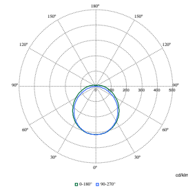
Polar Normal (separate) - 911401841185
