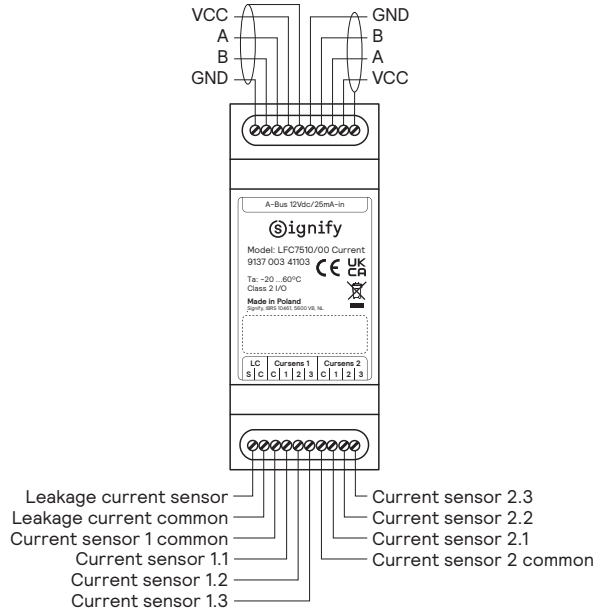
Current and leakage sensor connection
