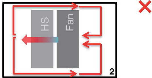
2. Design guidelines for active cooling solutions
