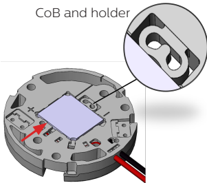
Step 3: Compress the spring with the CoB
