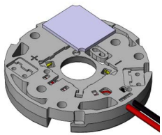
Step 1: Align the + and - of the CoB and holder
