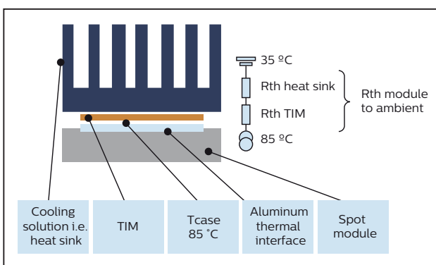
Thermal model
