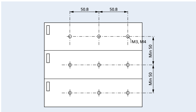
Mounting hole pattern for FastFlex 2x6 DA
