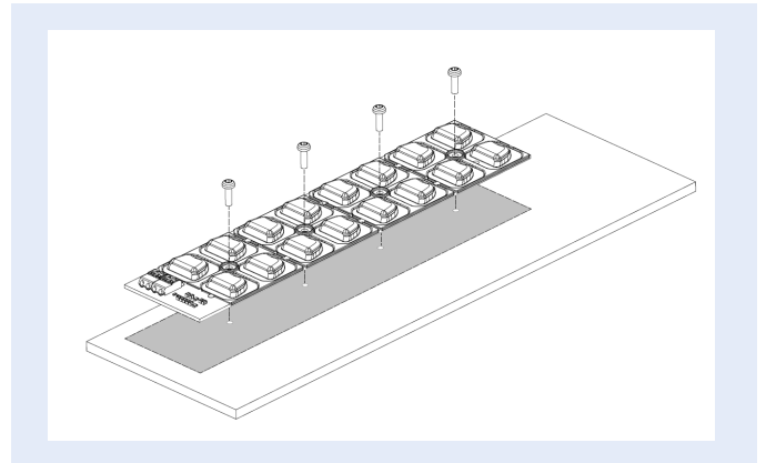
Example of fixation of the FastFlex module.
