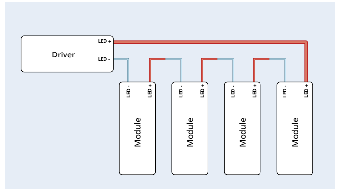
Example of connecting a Xitanium driver with multiple FastFlex DP or DHE LED modules
