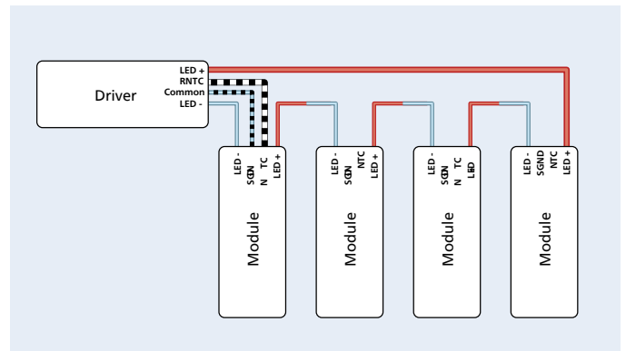
Example of connecting a Xitanium driver with multiple FastFlex DA LED modules. Connection of NTC is optional.
