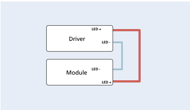
Example of connecting a Xitanium driver with a FastFlex DP or DHE LED module
