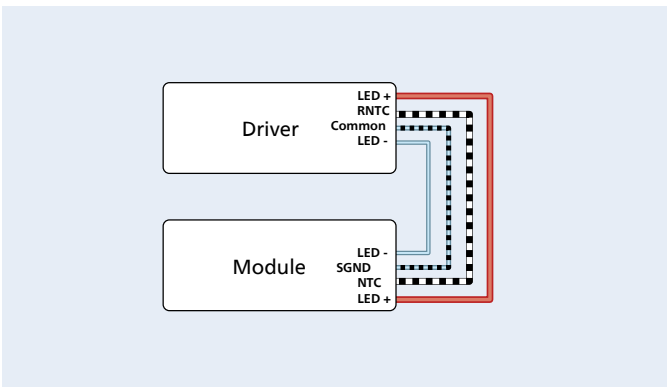
Example of connecting a Xitanium driver with a FastFlex DA LED module. Connection of NTC is optional.
