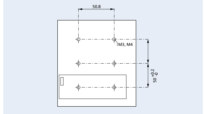
Mounting hole pattern for FastFlex 2x4 DA
