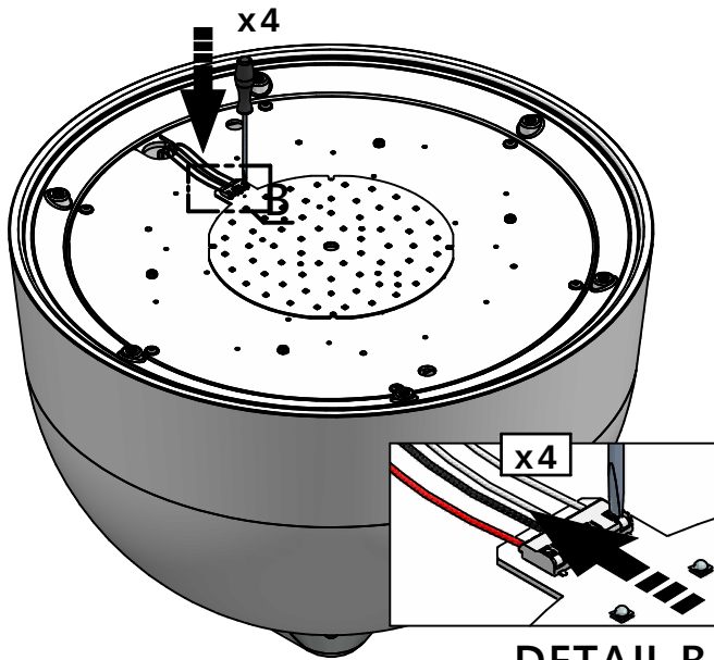
DETAIL B
