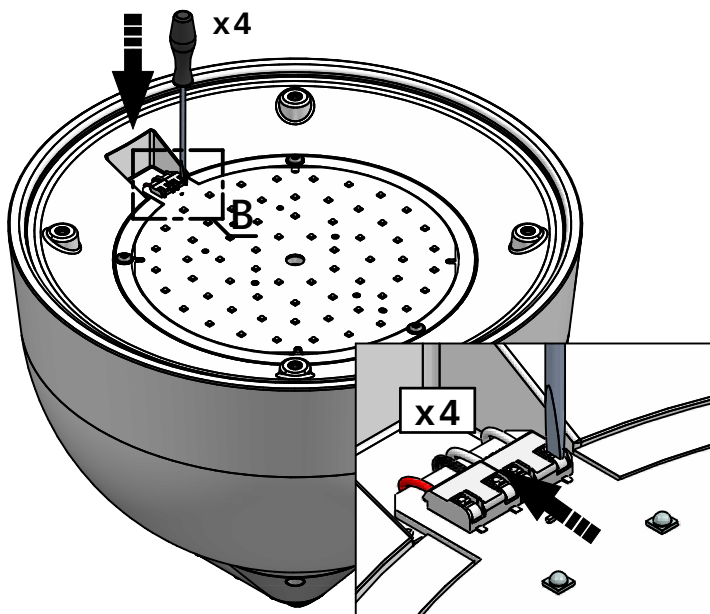
DETAIL B
