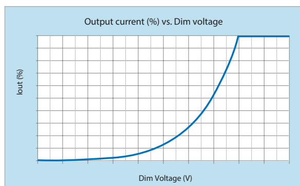
Figure 9. Output current in % vs dimming voltage (logarithmic dimming curve), example.
