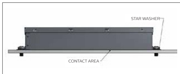
Figure 13. Chassis mounting.
