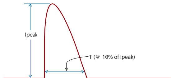
Figure 10. Inrush current vs. time.
