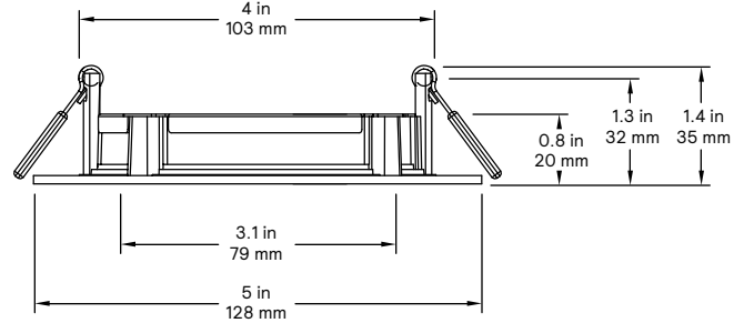
Downlight 4" Round
