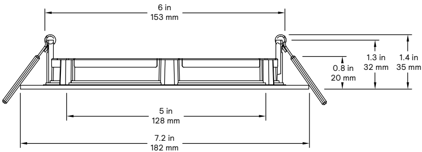
Downlight 6" Round
