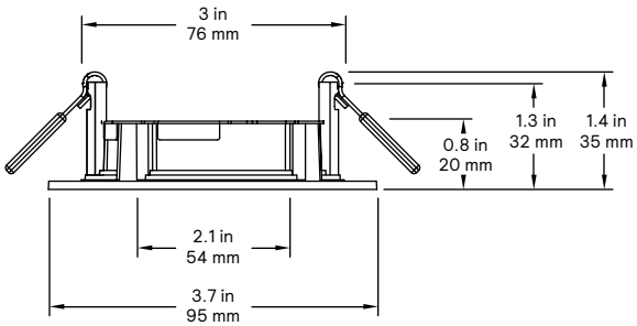
Downlight 3" Round
