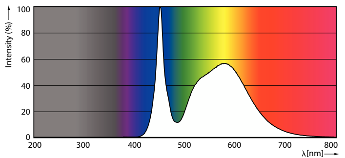
Spectral Power Distribution Colour - 180-130-100CC/LED/3PW/750/EX39 BB 3/1
