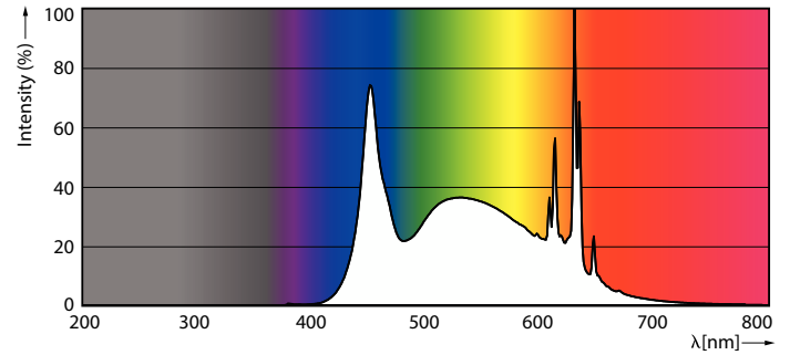
Spectral Power Distribution Colour - MAS LED spot VLE D 5.5-80W GU10 965 36D
