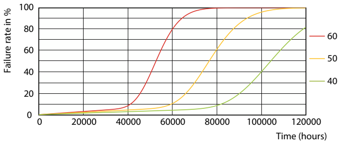
LEDtube_100K_4060_FailureRate-LED
