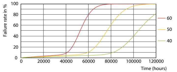
LEDtube_100K_4060_FailureRate-LED
