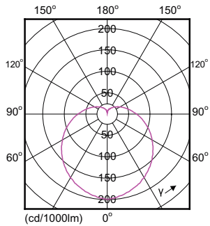
Light Distribution Diagram - EcoHome LEDBulb 14W E27 6500KLV 1PF/20
