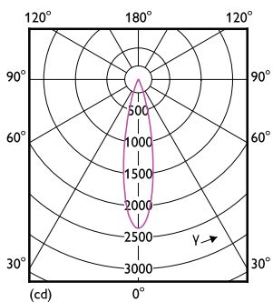
Light Distribution Diagram - RS280 G2 RC Rd D75 5W 30K 24D
