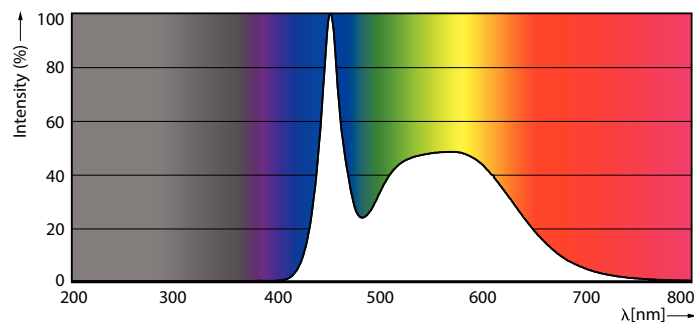
Spectral Power Distribution Colour - EcoHome LEDBulb 8W E27 6500KHV 2PF/10AR
