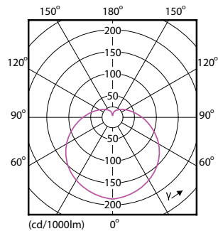
Light Distribution Diagram - EcoHome LEDBulb 8W E27 6500KHV 2PF/10AR
