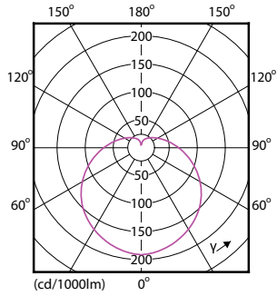
Light Distribution Diagram - EcoHome LEDBulb 6W E27 6500KHV 1PF/20UY
