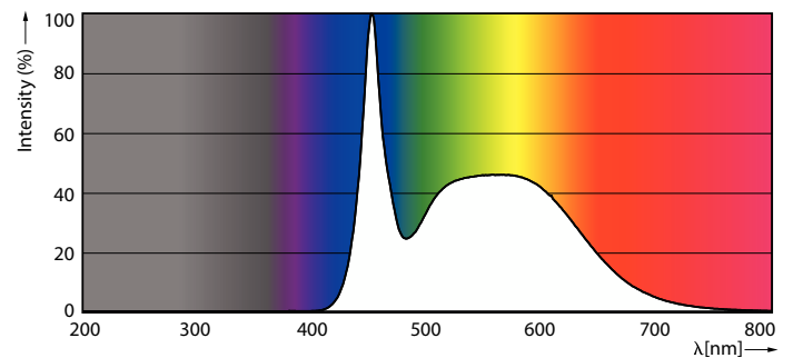
Spectral Power Distribution Colour - EcoHome LEDBulb 6W E27 6500KHV 1PF/20UY
