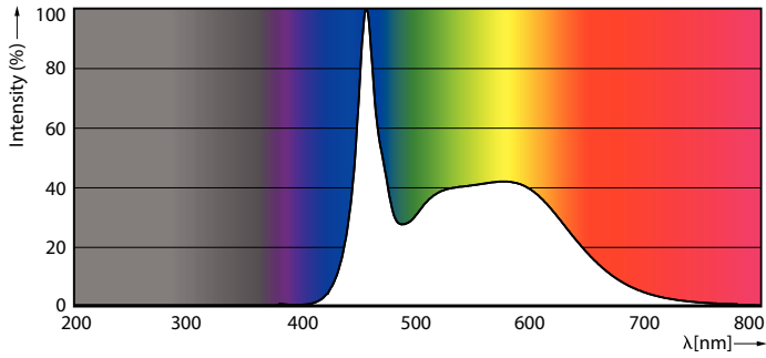
Spectral Power Distribution Colour - CorePro LEDspot 4.9-65W GU10 865 36D
