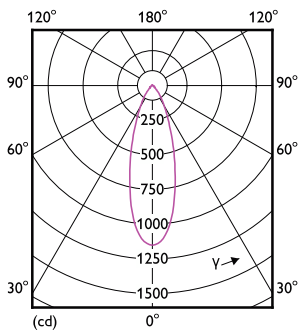
Light Distribution Diagram - CorePro LEDspot 4.9-65W GU10 865 36D
