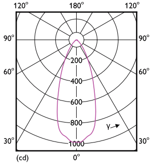
Light Distribution Diagram - 5.5PAR20/COR/F40/930/DIM/P/T20 6/1FB
