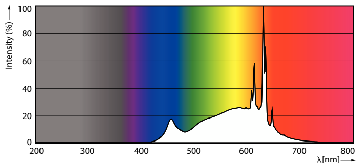
Spectral Power Distribution Colour - 5.5PAR20/COR/F40/930/DIM/P/T20 6/1FB
