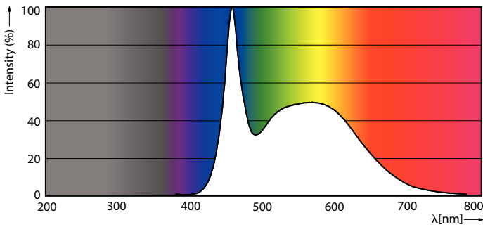
Spectral Power Distribution Colour - TForce ESS LED HB MV 4.5Klm 45W 865 E27
