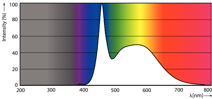
Spectral Power Distribution Colour - TForce ESS LED HB MV 2.5Klm 25W 865 E27
