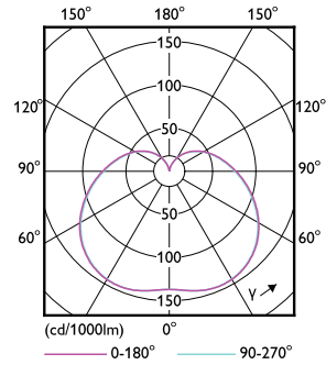
Light Distribution Diagram - TForce ESS LED HB MV 2.5Klm 25W 865 E27
