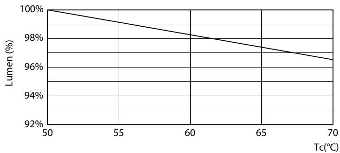
Lumen Maintenance Diagram - CorePro LEDtube 600mm 8W 865 VVW T8
