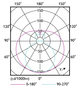
Light Distribution Diagram - CorePro LEDtube 1200mm 17W 865 T8 AU 1CT
