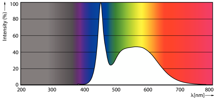
Spectral Power Distribution Colour - CorePro LEDtube 1200mm 17W 865 T8 AU 1CT
