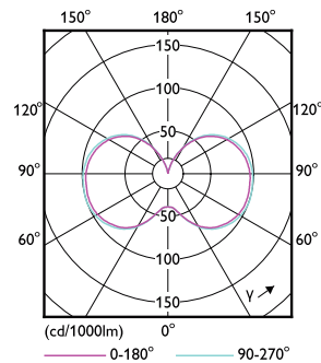
Light Distribution Diagram - 115CC/LED/850/LS EX39 G2 BB 277-480V 3/1
