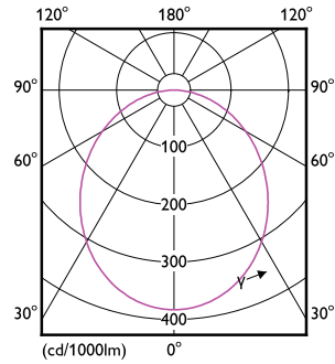
Light Distribution Diagram - DN020B G4 LED6/WW 6W 220-240V D125
