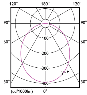
Light Distribution Diagram - DN020B G4 LED6/NW 7W 220-240V D100
