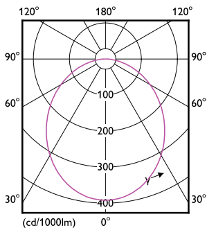
Light Distribution Diagram - DN200 G3 LED4 865 4.5W D90 CN
