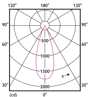
Light Distribution Diagram - RS350 G2 RC Rd D55 7W 40K 36D 1H
