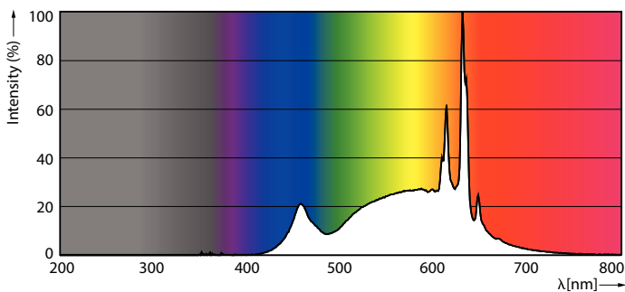
Spectral Power Distribution Colour - CorePro LEDbulb ND 13-100W A60 E27 930
