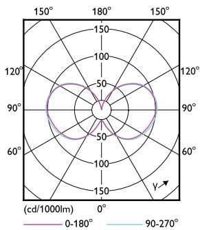
Light Distribution Diagram - 63CC/LED/840/LS EX39 G3 BB 3/1
