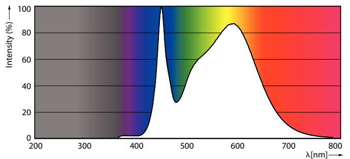
Spectral Power Distribution Colour - 45CC/LED/840/LS EX39 G3 BB 3/1
