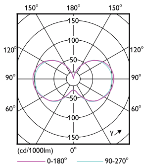
Light Distribution Diagram - 45CC/LED/840/LS EX39 G3 BB 3/1
