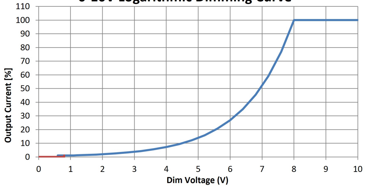
0-10V Logarithmic Dimming Curve
