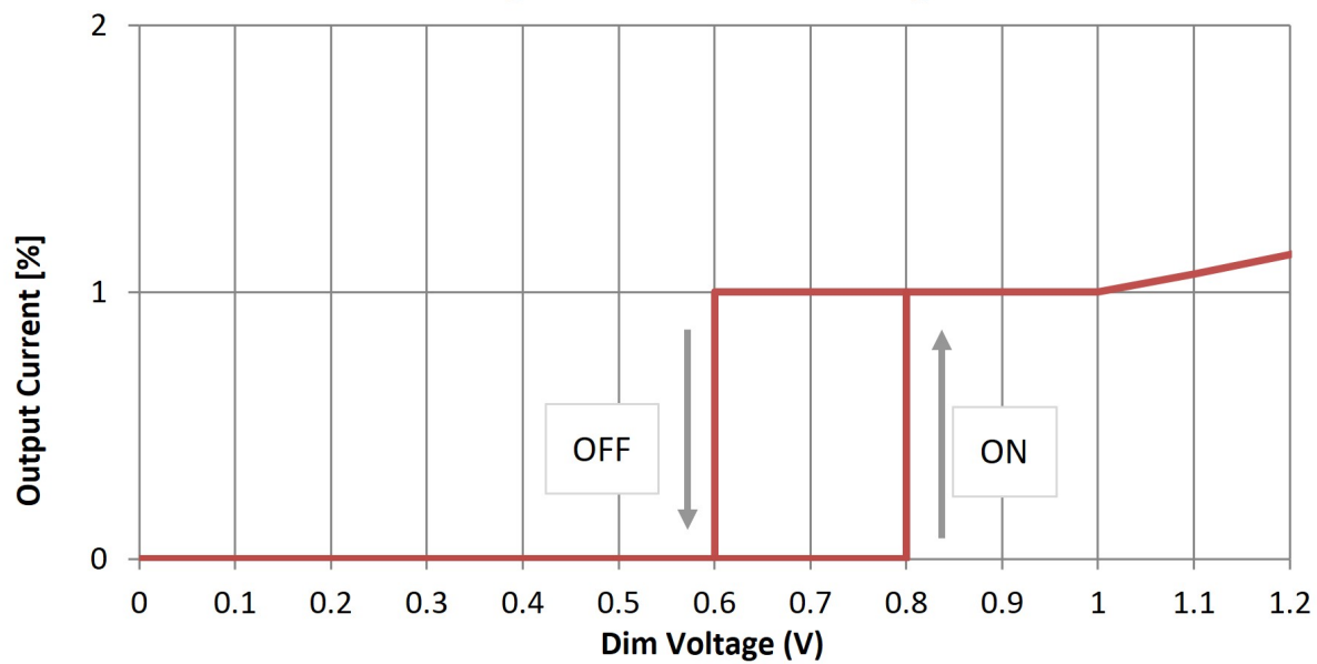
0-10V Logarithmic Dimming Curve
