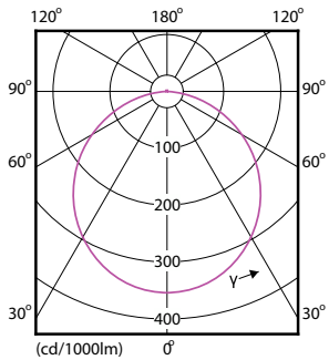
Light Distribution Diagram - DN027B G3 LED6/WW 6W 220-240V D90 RD
