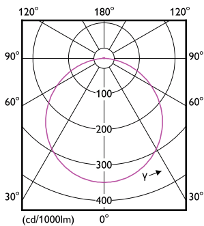
Light Distribution Diagram - DN020B G3 LED4/NW 4.5W 220-240V D90 GM
