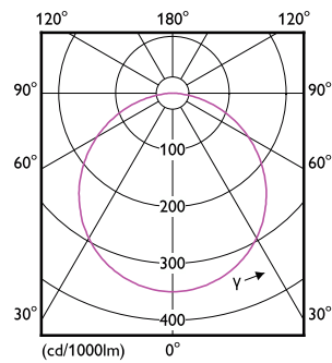
Light Distribution Diagram - DN020B G3 LED3/CW 3.5W 220-240V D80 GM
