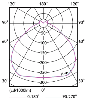
Light Distribution Diagram - 165HB/LED/850/D WB UDL BB G2 4/1
