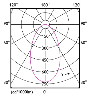
Light Distribution Diagram - 145HB/LED/840/D NB DL BB G2 4/1
