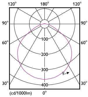
Light Distribution Diagram - TForce HB 160W E39 850 WB JP
