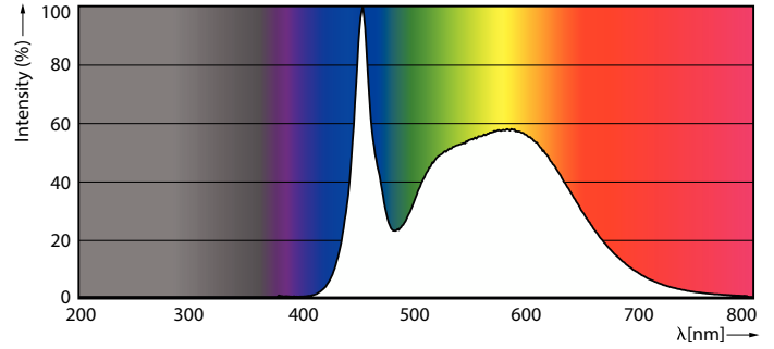
Spectral Power Distribution Colour - TForce HB 160W E39 850 WB JP
