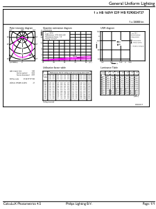
General uniform lighting - TForce HB 160W E39 850 WB JP
