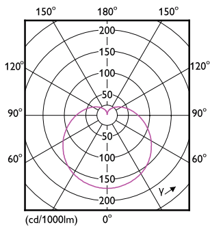
Light Distribution Diagram - LEDBulb 18W E27 6500K W A70 1PF/6 BR
