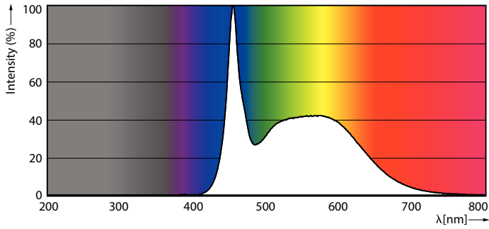
Spectral Power Distribution Colour - LEDBulb 18W E27 6500K W A70 1PF/6 BR
