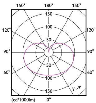
Light Distribution Diagram - LED Sensor 8W B22 WH FR 1PF/6 APR
