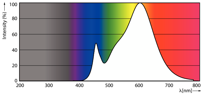
Spectral Power Distribution Colour - LED Sensor 8W B22 WH FR 1PF/6 APR
