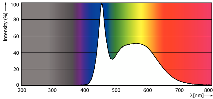
Spectral Power Distribution Colour - EcoHome LEDBulb 10W E27 6500KLV 1PF/12MX
