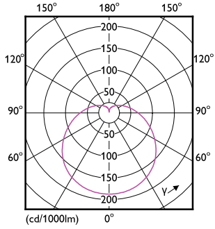
Light Distribution Diagram - EcoHome LEDBulb 10W E27 6500KLV 1PF/12MX
