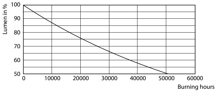
Lumen Maintenance Diagram - MAS LED spot VLE D 650lm GU10 930 120D
